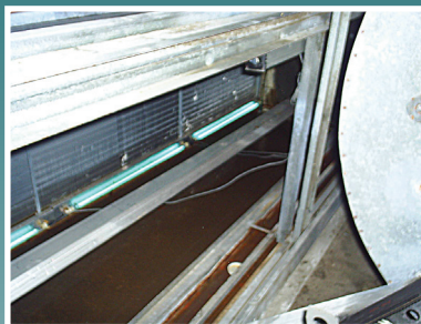
Air Handler with Fresh-Aire TM Commercial Series UV Lights Installed
